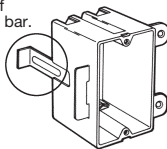
Proper mounting position of stabilizing bar.
