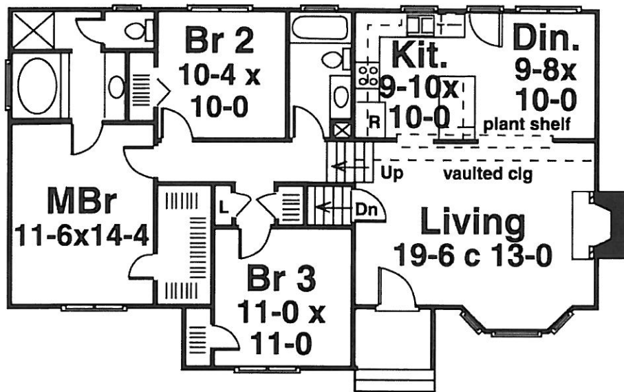
SECOND FLOOR
