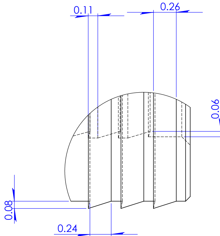
DETAIL A SCALE 2 : 1.25
